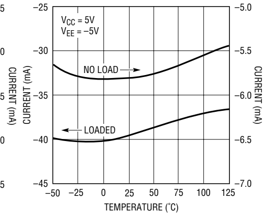
I_{EE} Supply Current vs Temperature
