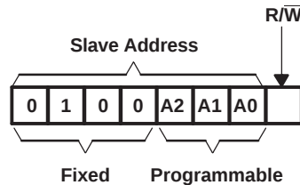
Figure 22. PCA9555 Address
