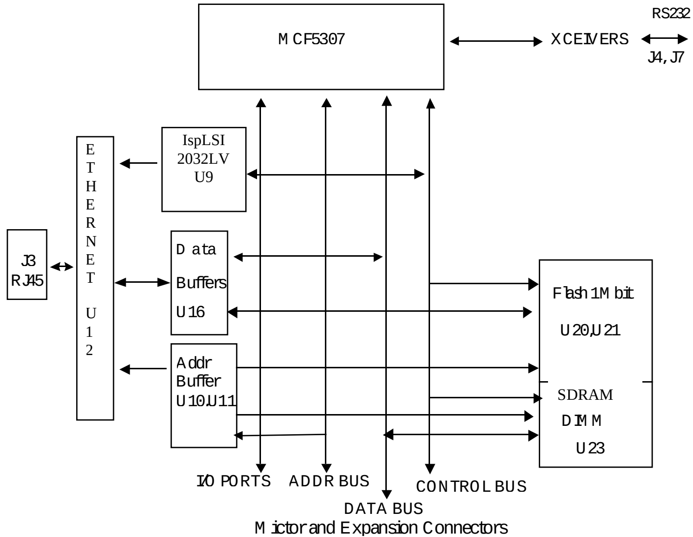
Figure 1 Block Diagram of the board
