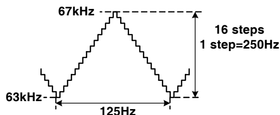
Figure 20. Frequency Modulation
