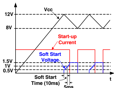
Figure 19. Start-up Current and Vcc Voltage
