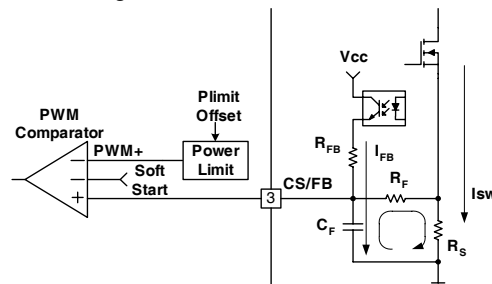
Figure 21. Current Sense and Feedback Circuits
