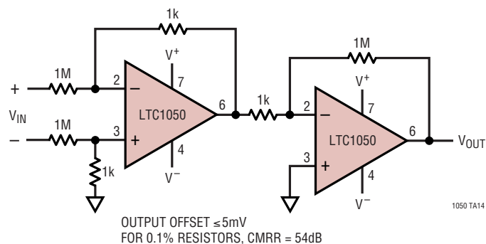
Instrumentation Amplifier with 100V Common Mode Input Voltage
