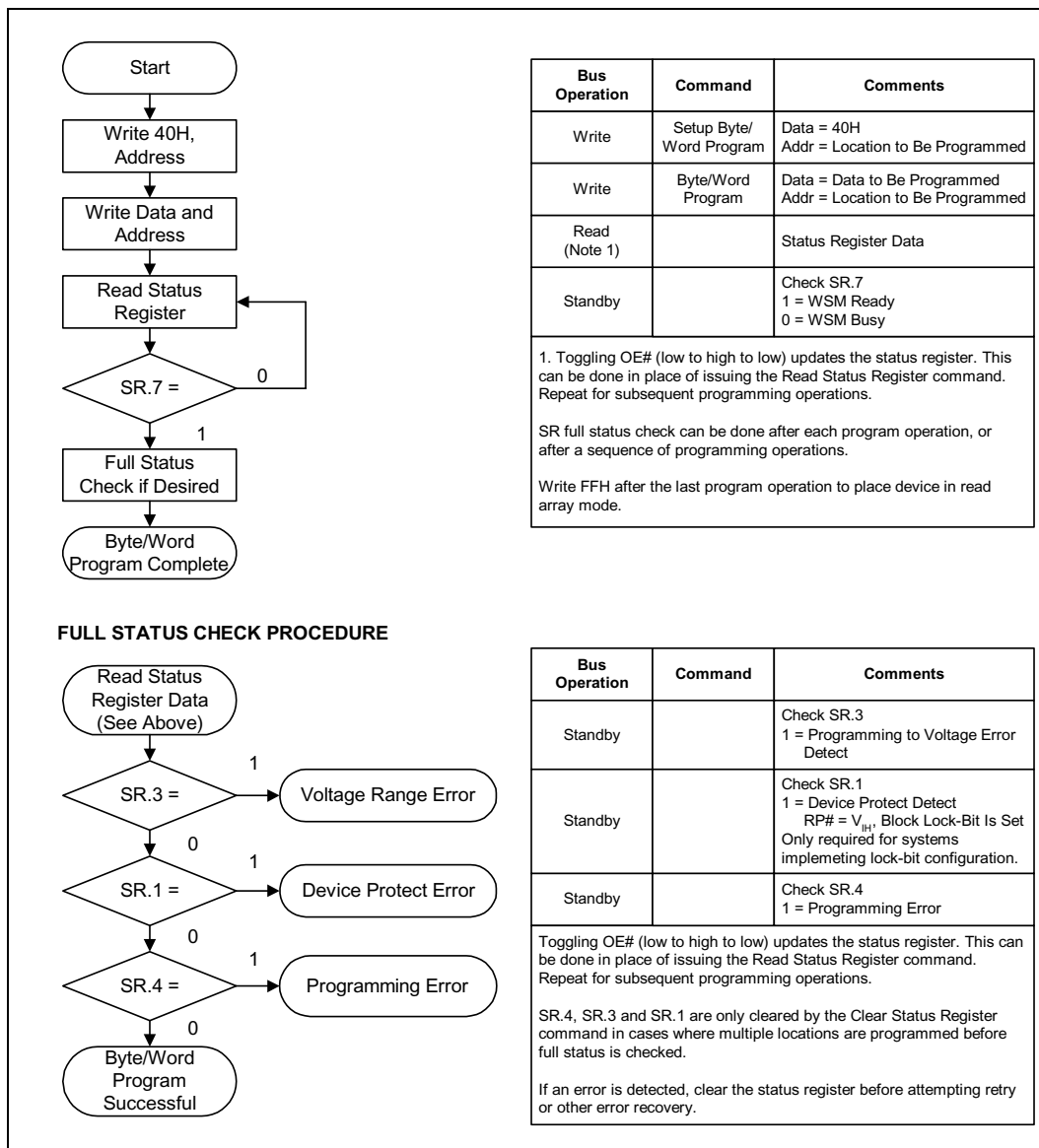
Figure 7. Byte/Word Program Flowchart
