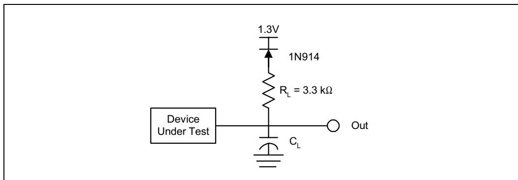
Figure 14. Transient Equivalent Testing Load Circuit
