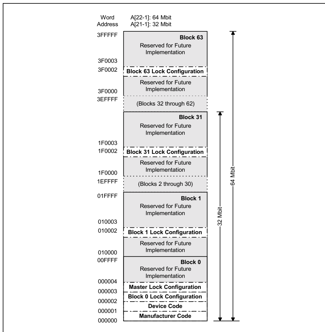
Figure 5. Device Identifier Code Memory Map
