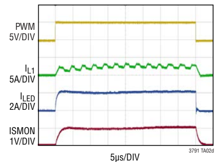
100Hz 250:1 PWM Dimming ( V_{IN} = 24V )
