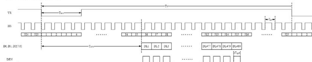
RGB Mode (1920X480) Vertical Timing
