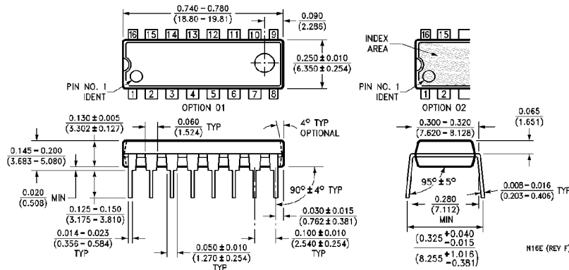
Molded Dual-In-Line Package (N) Order Number CD4028BMN or CD4028BCN NS Package Number N16E
