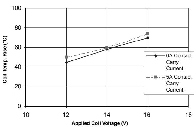
Overcurrent Energization (85°C, G8N-1 225Ω coil, 4 samples)
