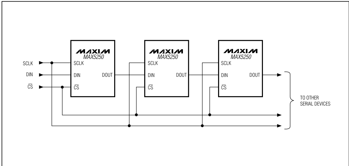
Figure 7. Daisy-Chaining MAX5250s
