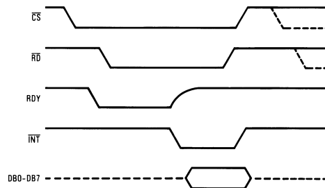
Figure 20. RD Mode (Pin 7 is Low)
