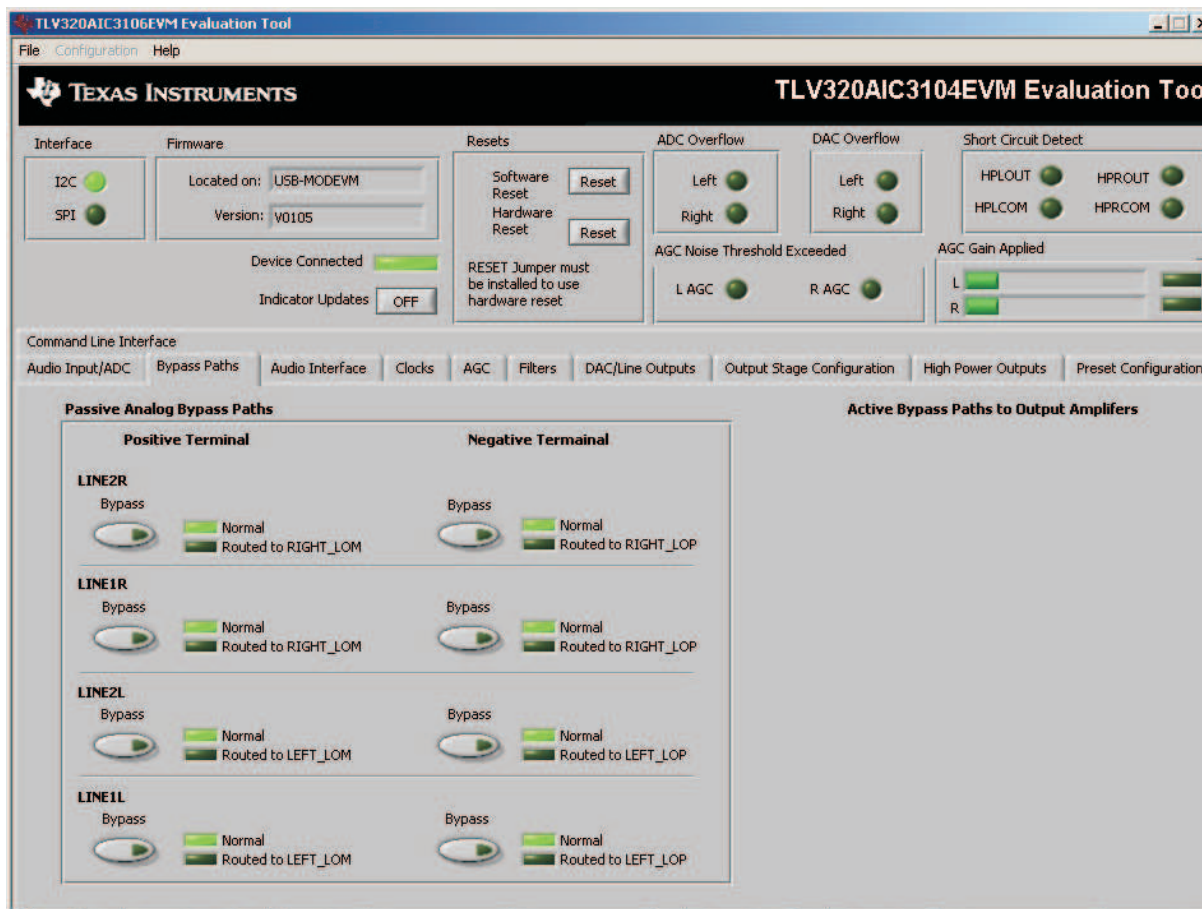
Figure 8. Bypass Paths
