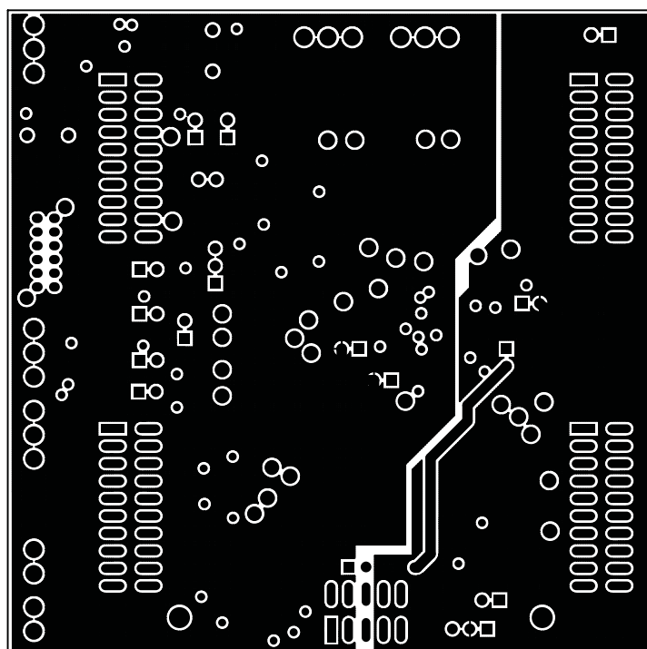
Figure 35. TLV320AIC3104EVM Layer 4
