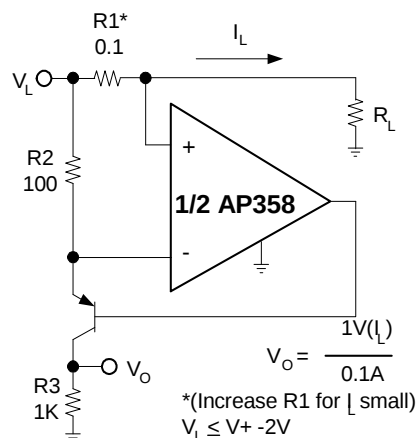
Current Monitor
