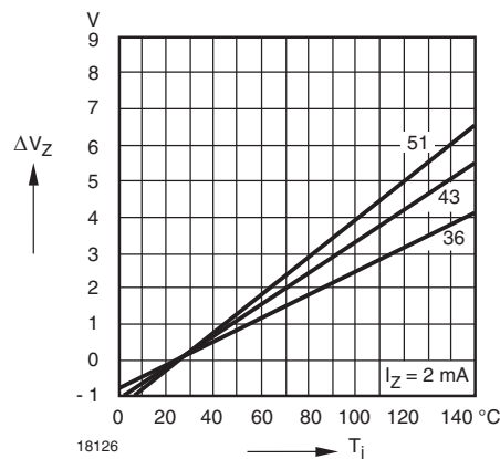
Fig. 11 - Change of Zener Voltage vs. Junction Temperature
