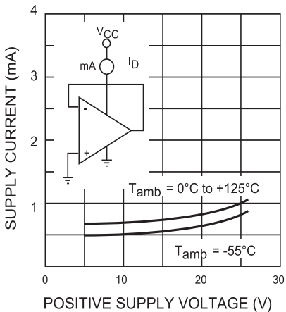
Figure 12. Supply current
