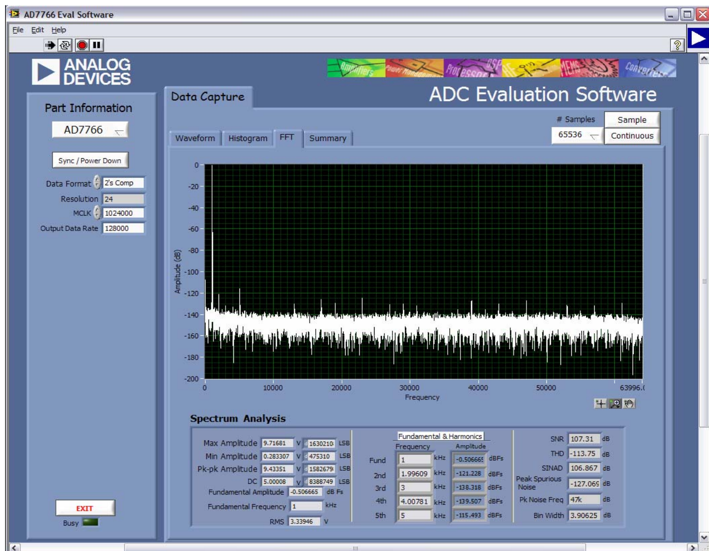
Figure 8. Data Capture AD7766/AD7766-1/AD7766-2 tab.
