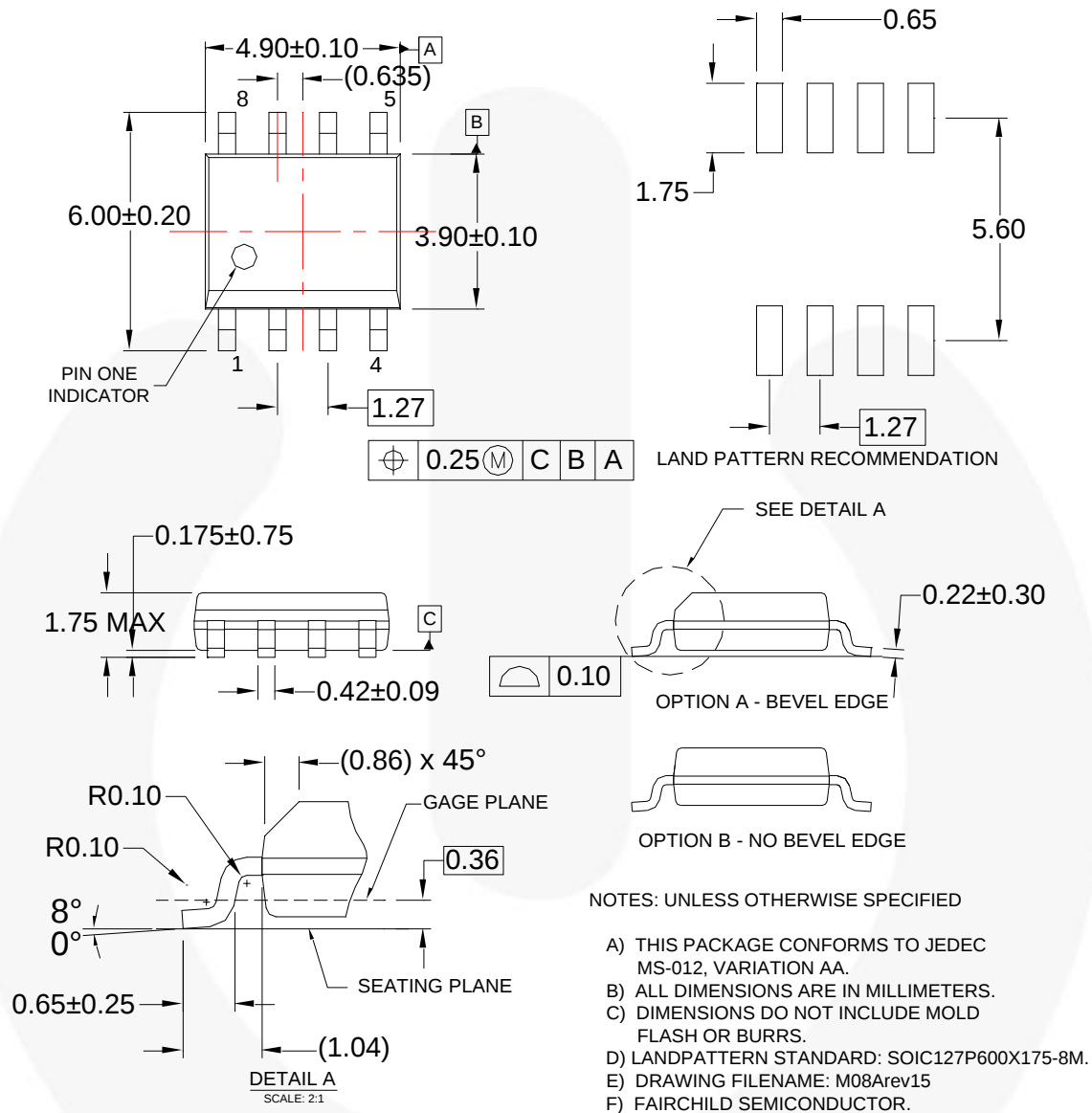
Figure 16. 8-Lead, Small Outline Package (SOP)
