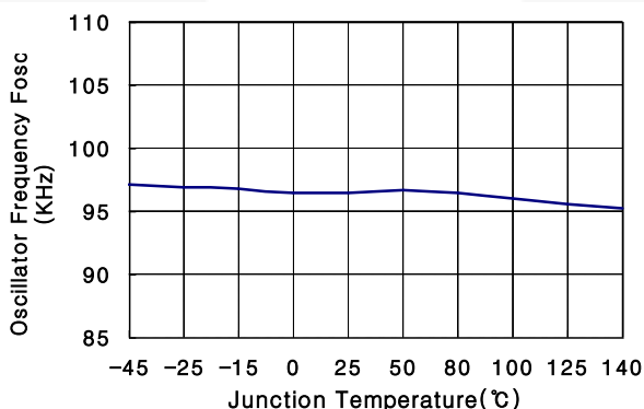
Figure 7. Oscillator Frequency
