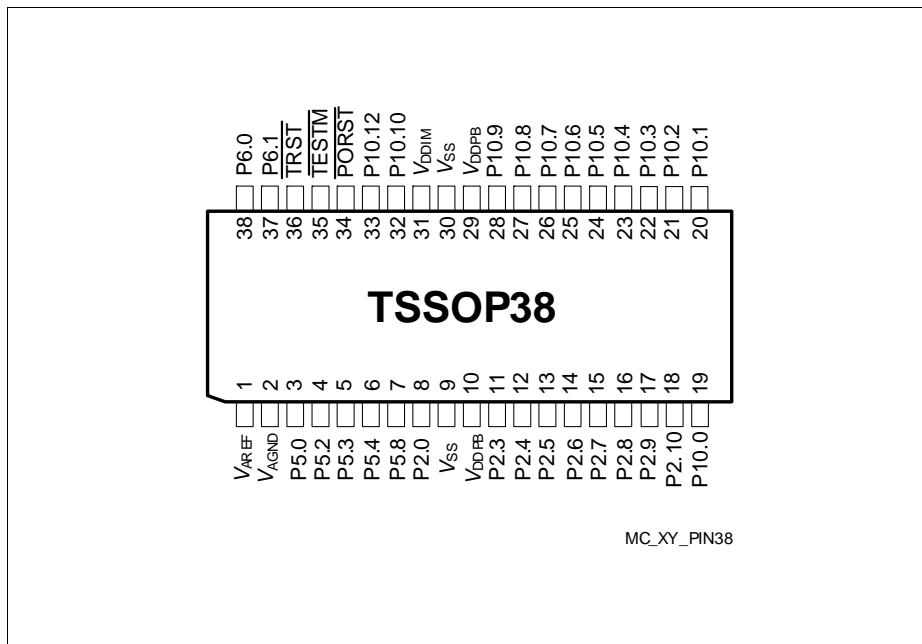
Figure 2 XC2712X Pin Configuration (top view)
