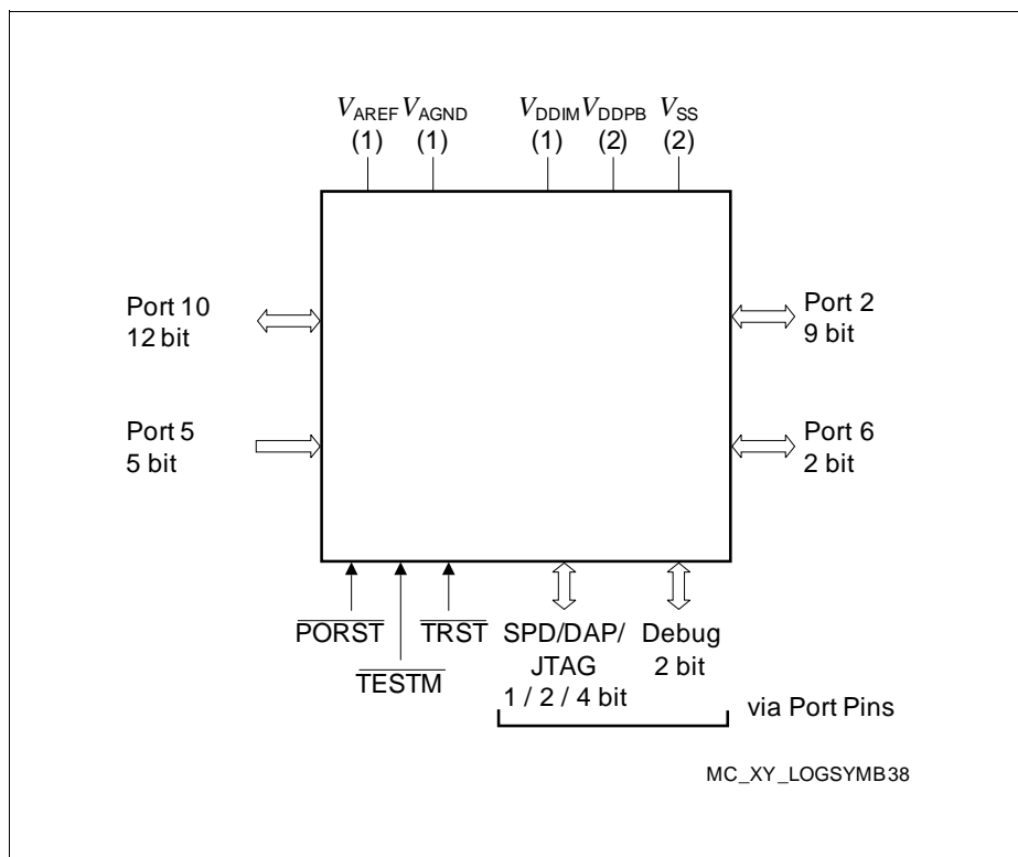
Figure 1 XC2712X Logic Symbol
