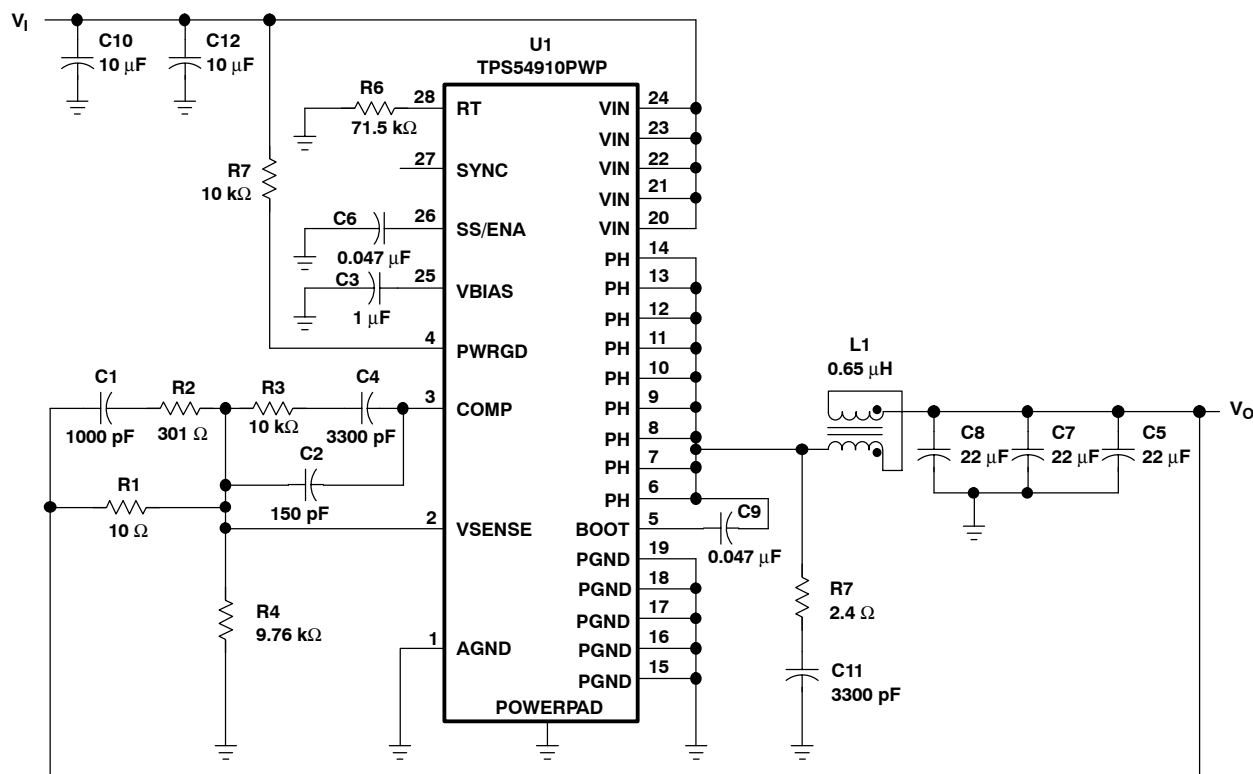
Figure 10. Application Circuit
