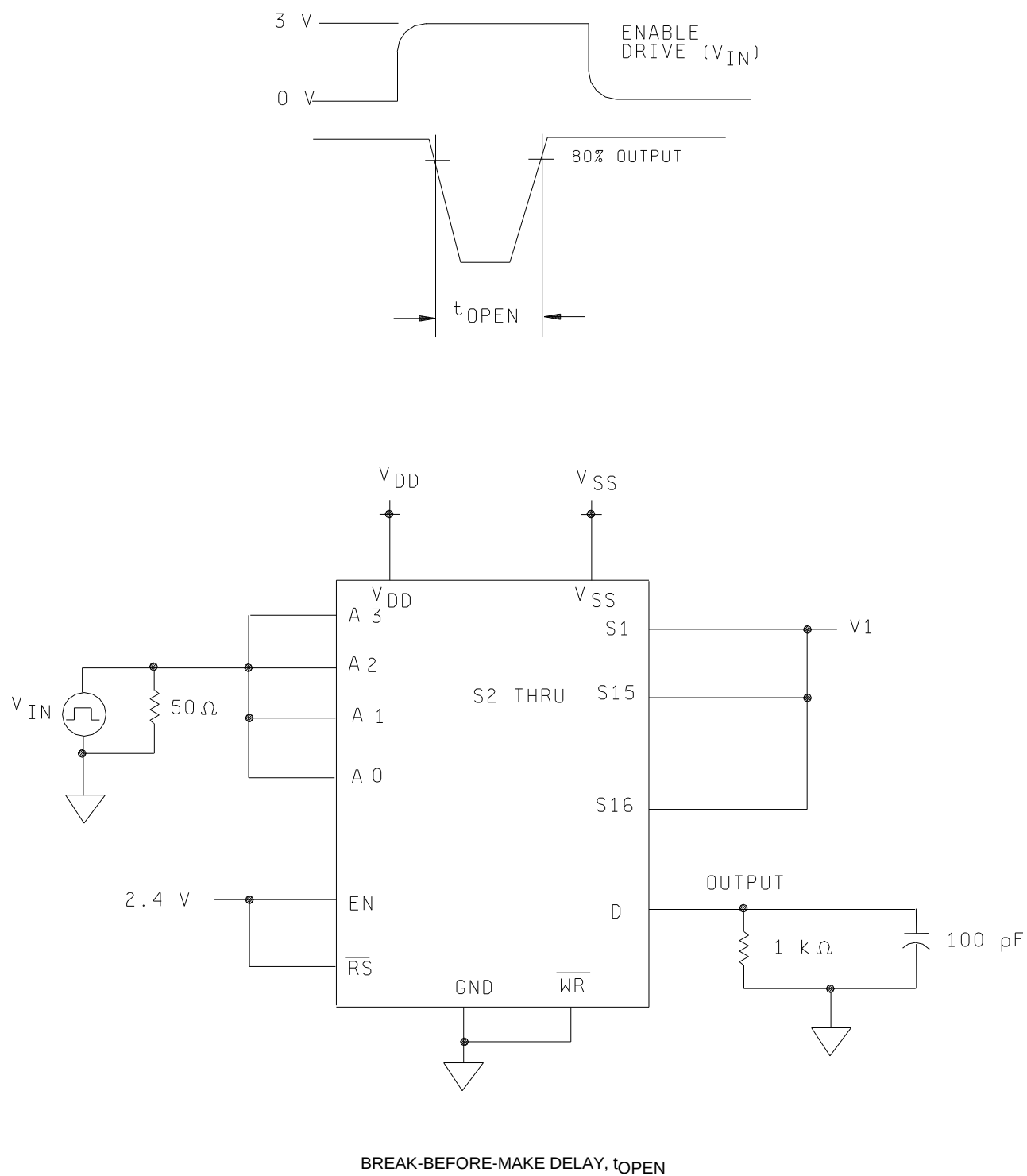
FIGURE 3. Test circuits.
