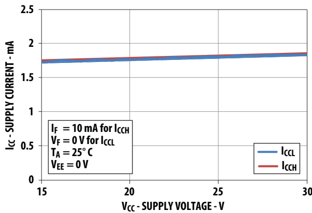
Figure 5. I_{CC} vs. V_{CC}
