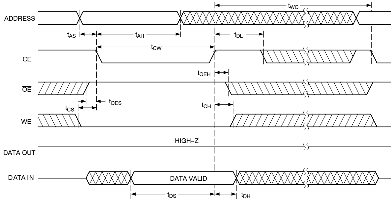
Figure 6. Byte Write Cycle [ \overline{\text{CE}} Controlled]
