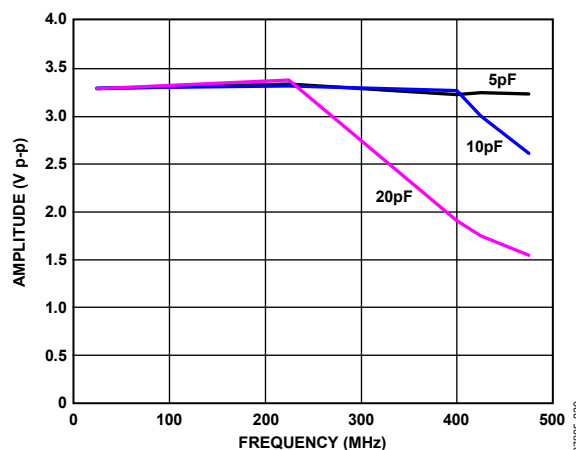
Figure 14. Peak-to-Peak Output Voltage vs. Frequency—CMOS
