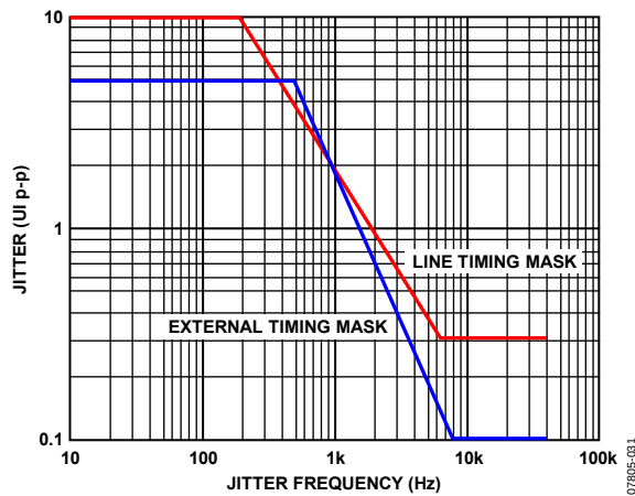
Figure 22. Jitter Tolerance
