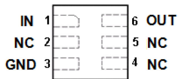
Figure 3. Pin Description
