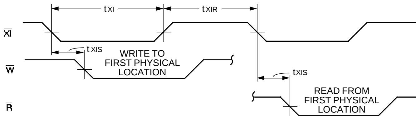
Figure 14. Expansion-In
