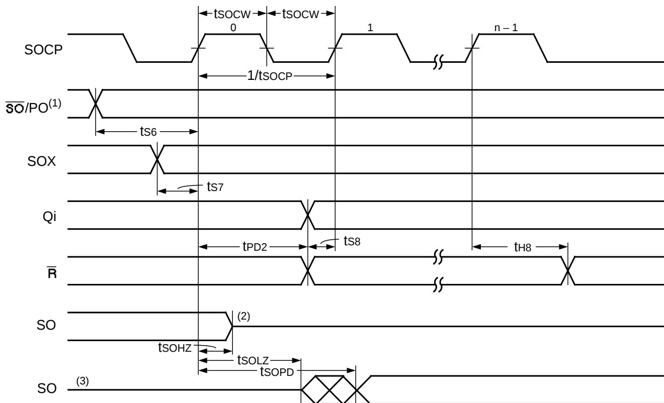
Figure 19. Write Operation In Serial-In Mode
