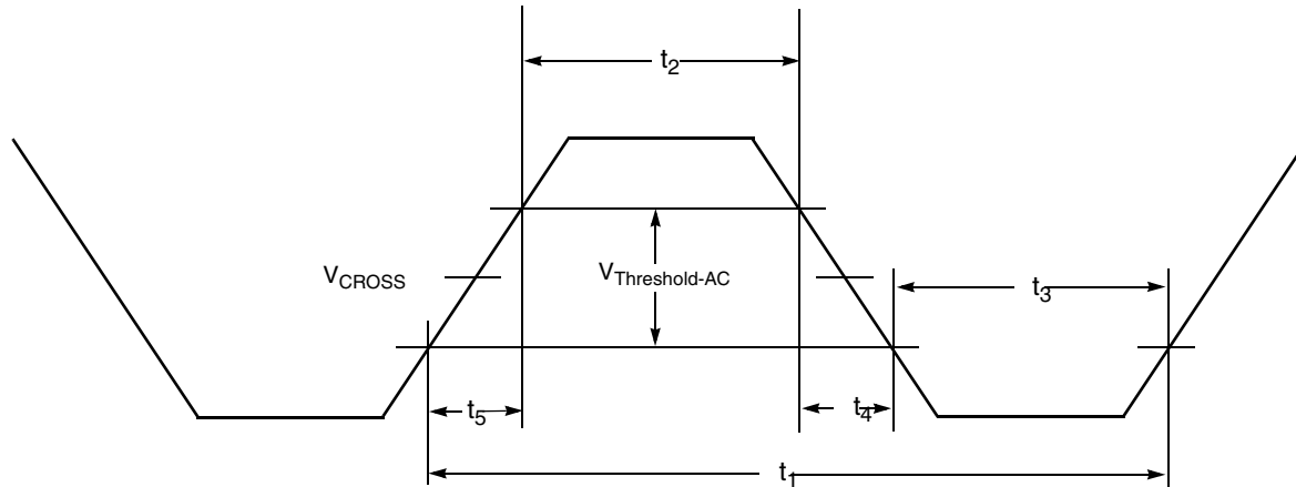
Figure 5-3. SYCLK Waveform
