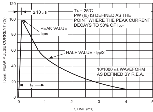
FIG.11- PULSE WAVEFORM
