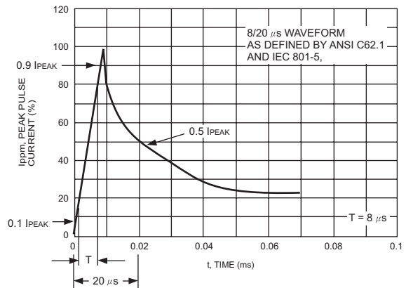
FIG.12- PULSE WAVEFORM
