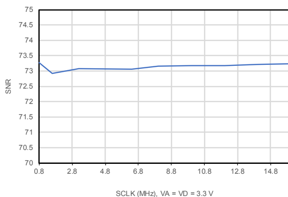
Figure 26. SNR vs. SCLK frequency
