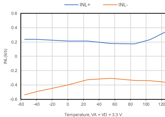
Figure 20. INL vs. temperature
