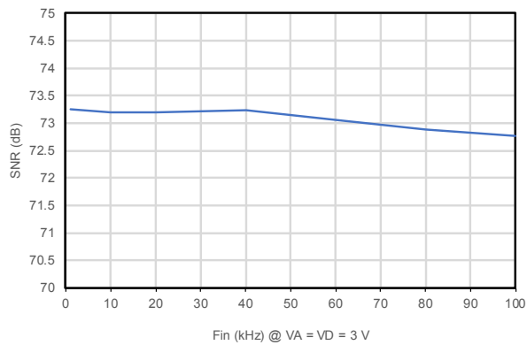
Figure 10. SNR vs. input frequency
