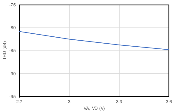
Figure 17. THD vs. power supply
