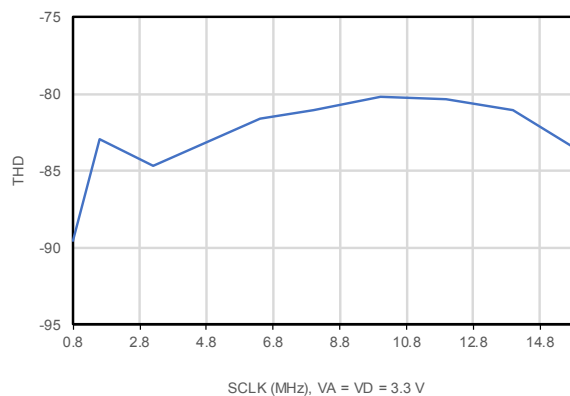
Figure 27. THD vs. SCLK frequency
