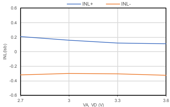
Figure 15. INL vs. power supply
