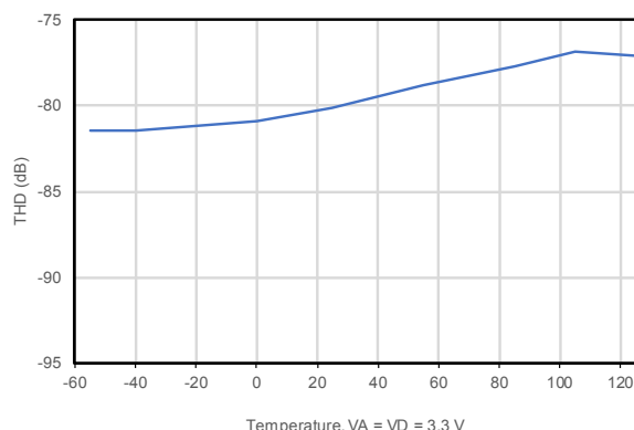
Figure 22. THD vs. temperature
