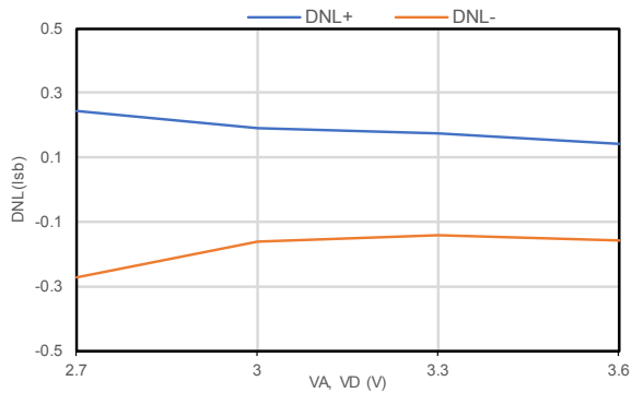
Figure 14. DNL vs. power supply
