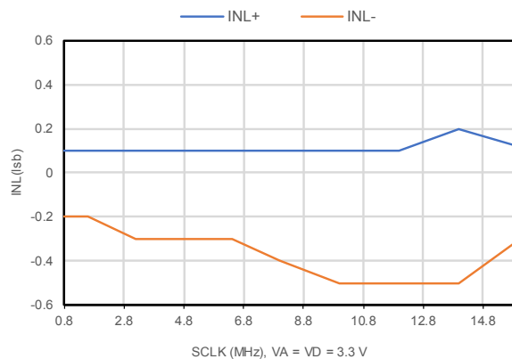
Figure 25. INL vs. SCLK frequency
