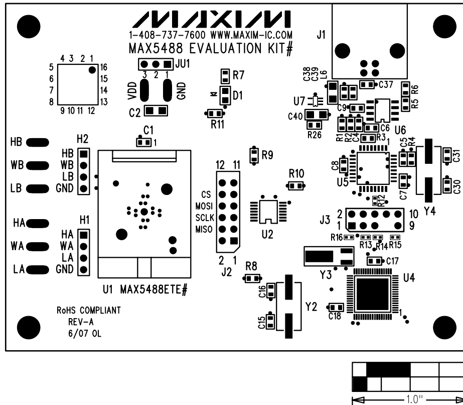
Figure 3. MAX5488 EV Kit Component Placement Guide—Component Side
