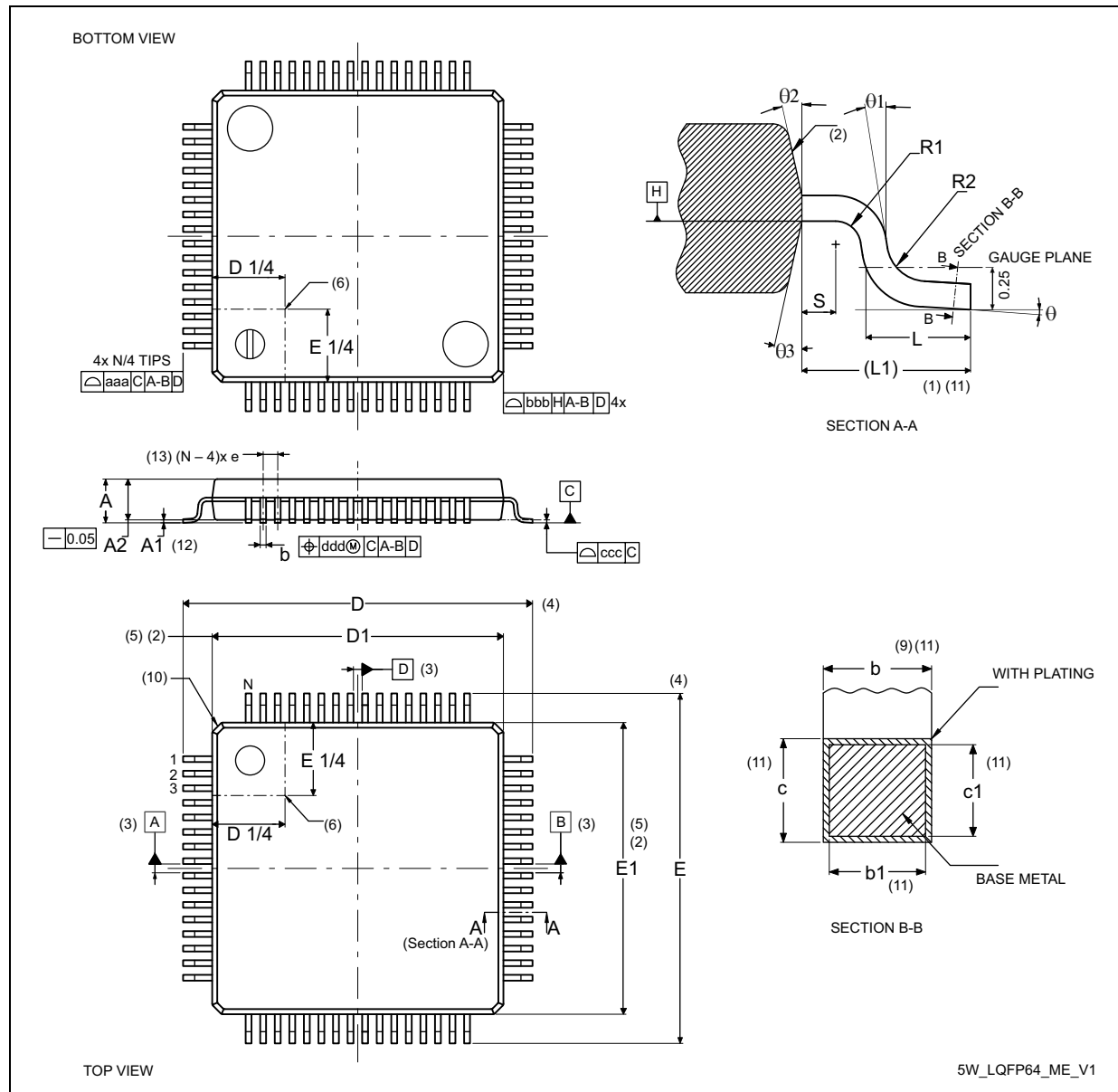
Figure 28. LQFP64 - Outline (15)
