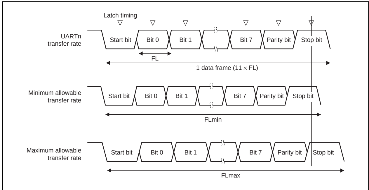
Figure 16-18. Allowable Baud Rate Range During Reception
