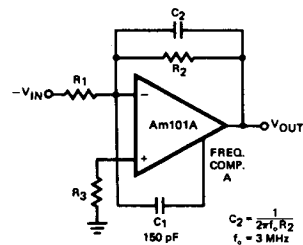
Feedforward Compensation
