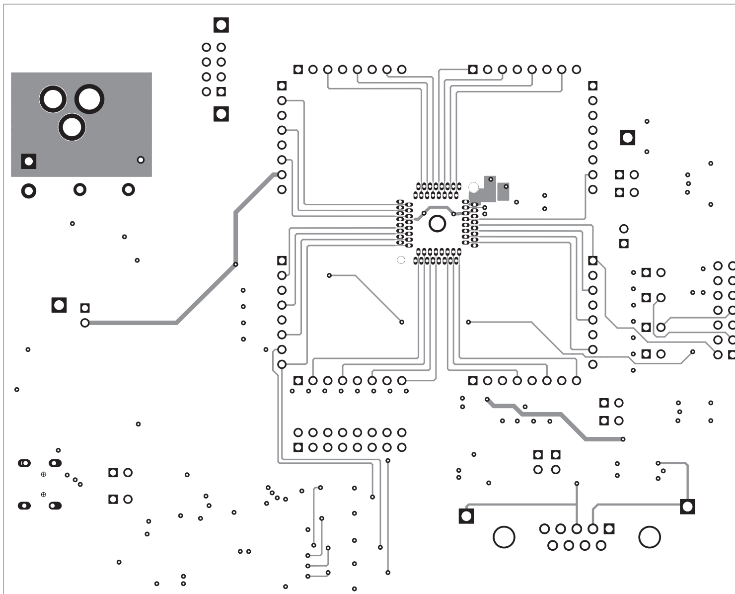
Figure 6. Layer-3 Routing
