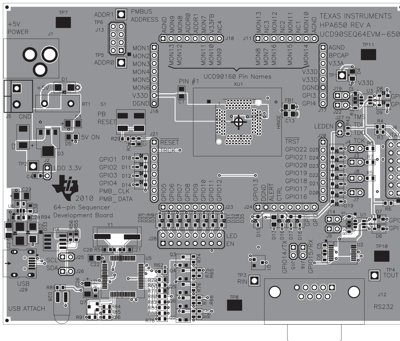
Figure 4. Top-Side Layout/Routing
