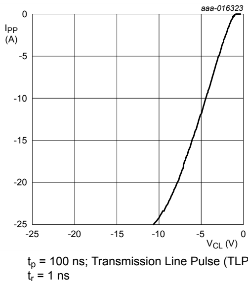
Fig. 10. Dynamic resistance with negative clamping; typical values
