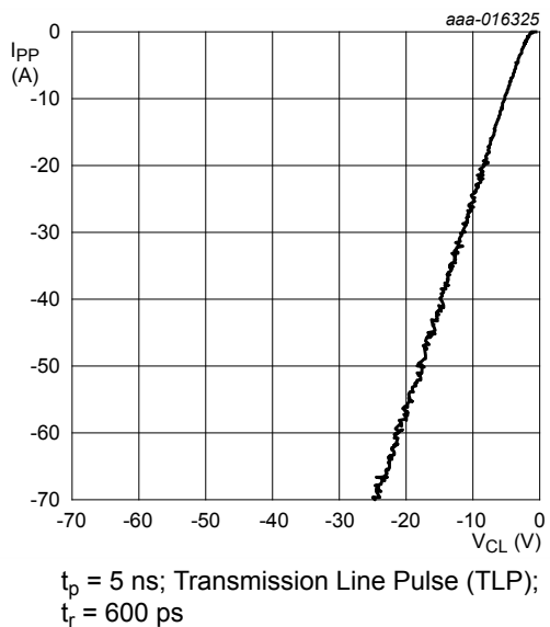
Fig. 12. Dynamic resistance with negative clamping; typical values
