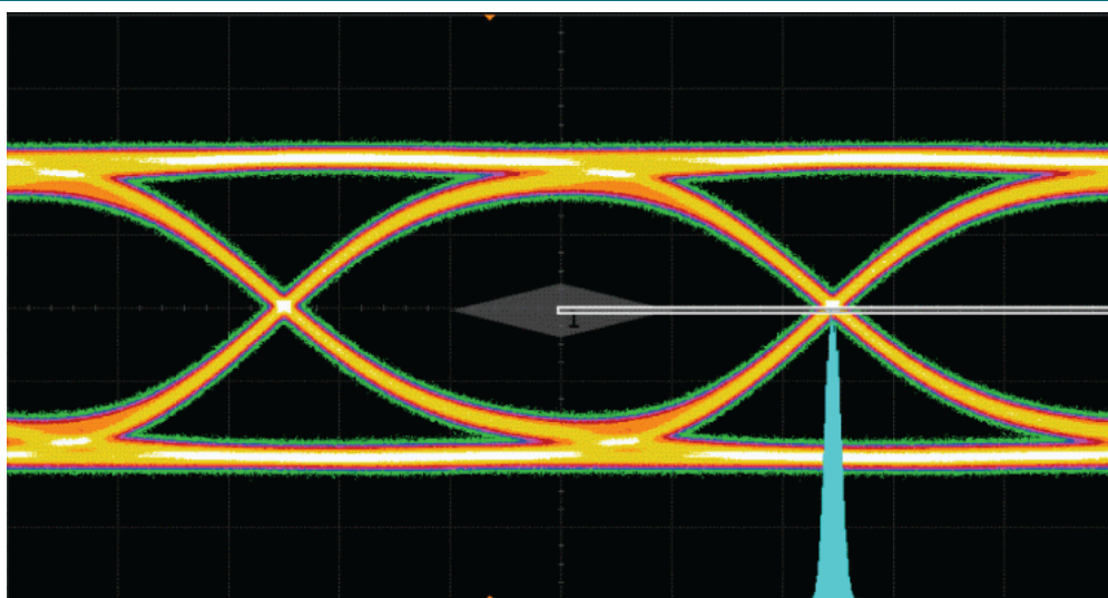
Fig. 7. HDMI 2.0 TP1 eye diagram, PCB with device
