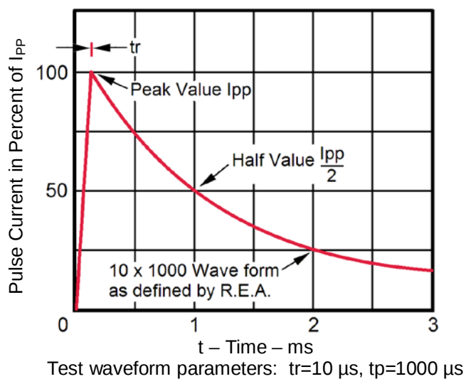
FIGURE 2 Pulse Waveform for 10/1000 \mu\text{s} Exponential Surge
