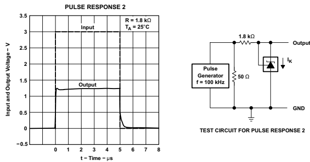
Figure 5-13. Pulse Response 2
