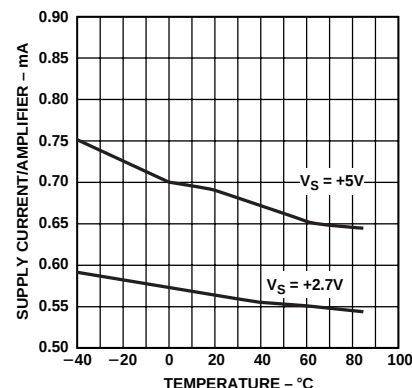
Figure 3. Supply Current per Amplifier vs. Temperature
