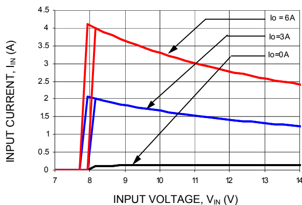
Figure 7. Input voltage vs. Input Current (V out = 5Vdc).
