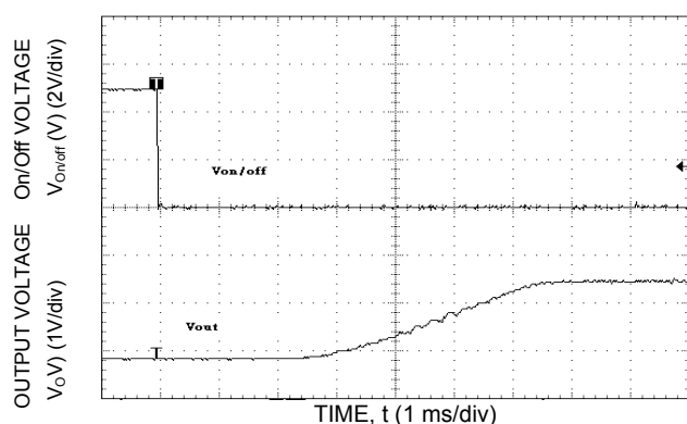
Figure 15. Typical Start-Up Using Remote On/Off with Low-ESR external capacitors (7x150uF Polymer) ( V_{in} = 12 Vdc, V_o = 3.3 Vdc, I_o = 6.0 A, C_o = 1050 \mu F).
