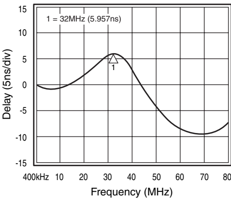
Figure 9. Group Delay vs. Frequency
