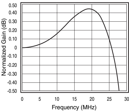
Figure 8. HD Gain Flatness
