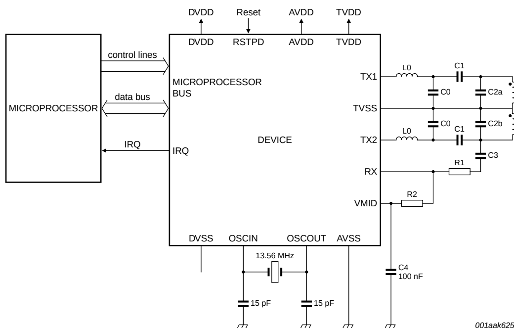
Fig 27. Application example circuit diagram: directly matched antenna
