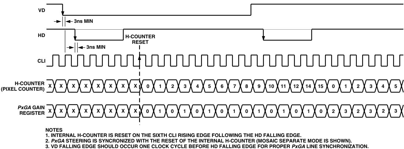
Figure 13. H-Counter Synchronization
