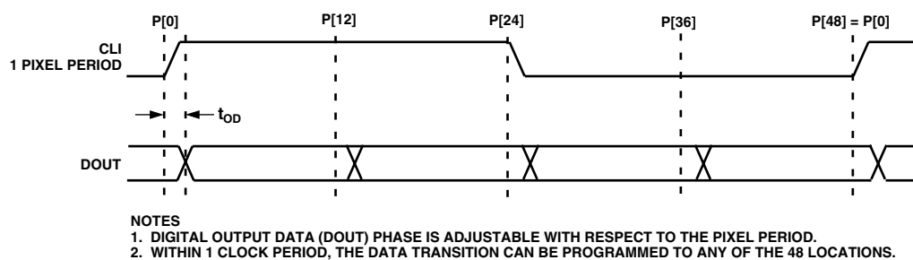
Figure 8. Digital Output Phase Adjustment
