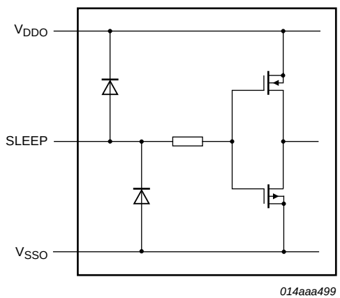
Fig 12. SLEEP 3-state input
