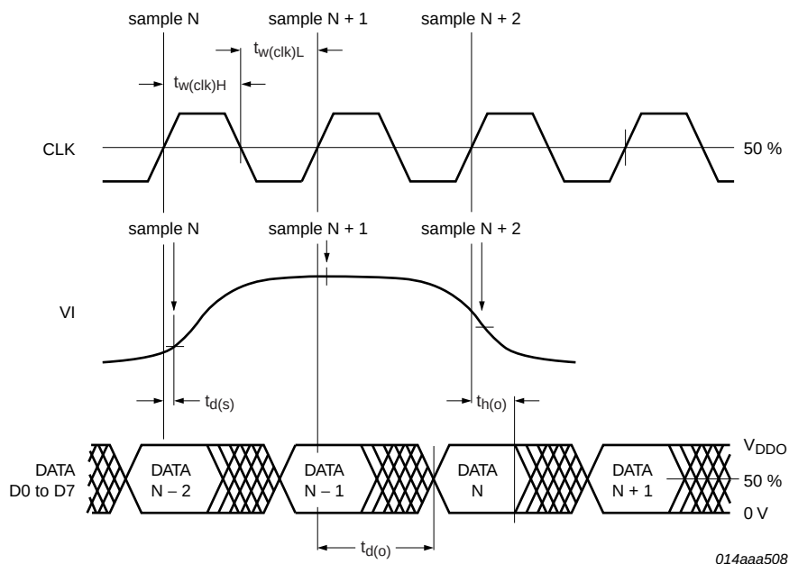
Fig 4. Timing diagram
