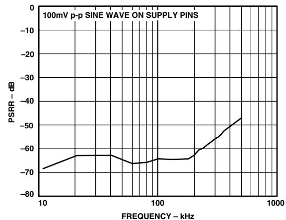
TPC 5. PSRR without Decoupling
