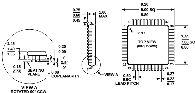
Figure 1. 48-Lead Low Profile Quad Flatpack [LQFP] 7 mm × 7 mm, Very Thin Quad (ST-48)
