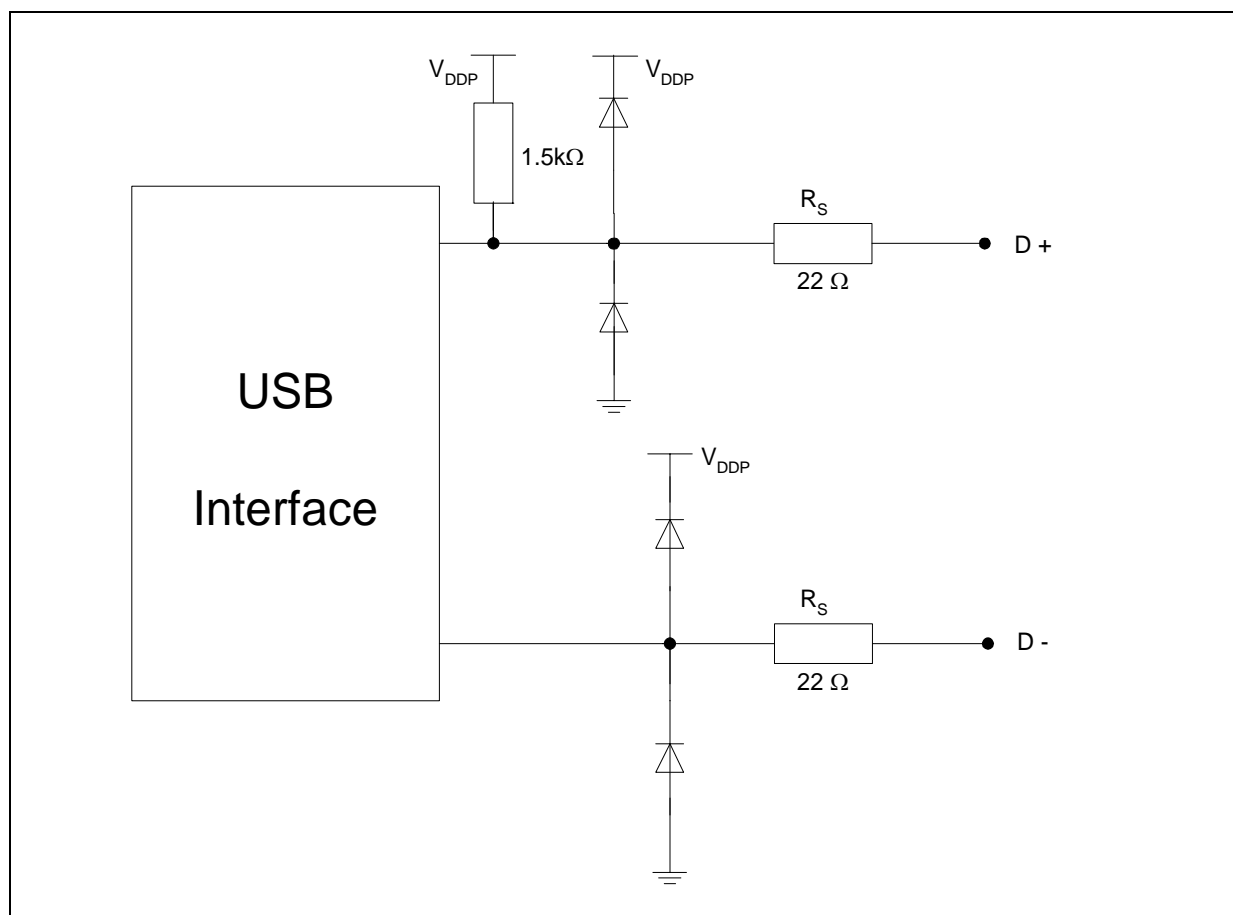
Figure 4-1 USB Interface
