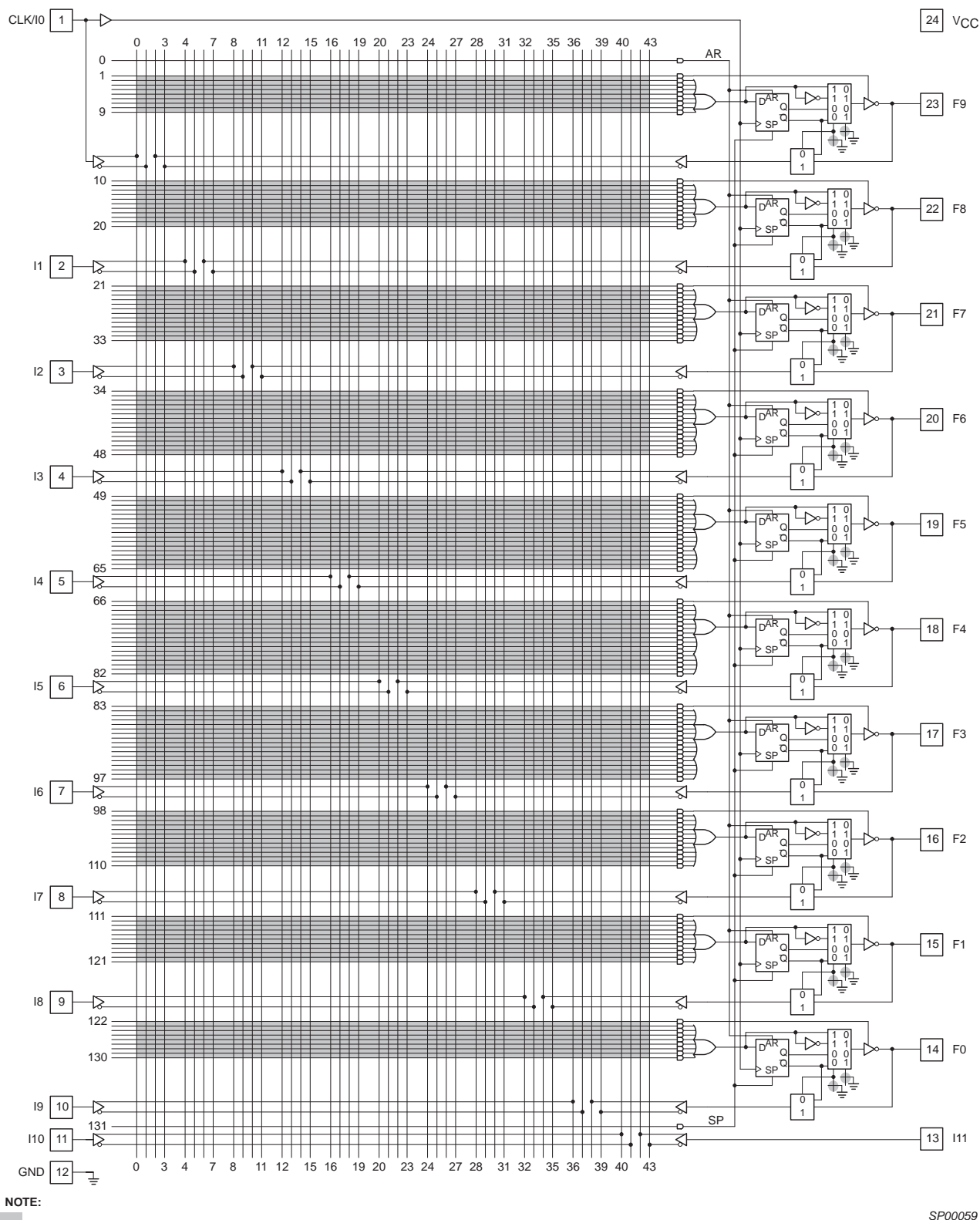
Figure 1: XCR22V10 Logic Diagram
