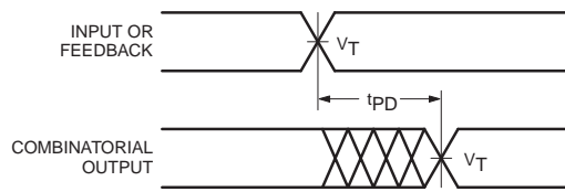
Combinatorial Output
