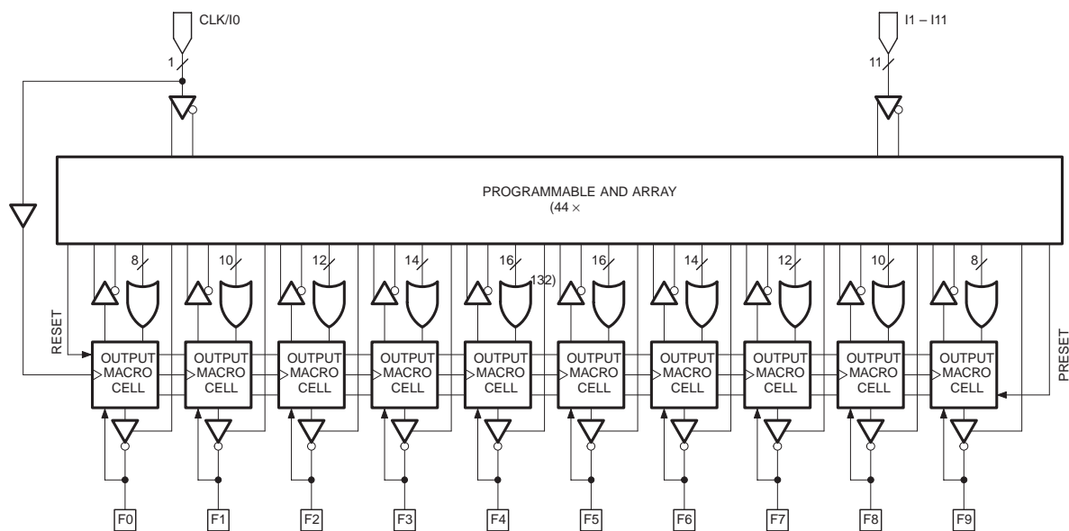
Figure 2: Functional Diagram
