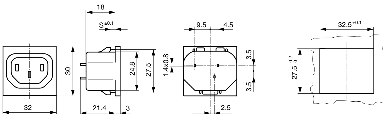
Appliance outlet
