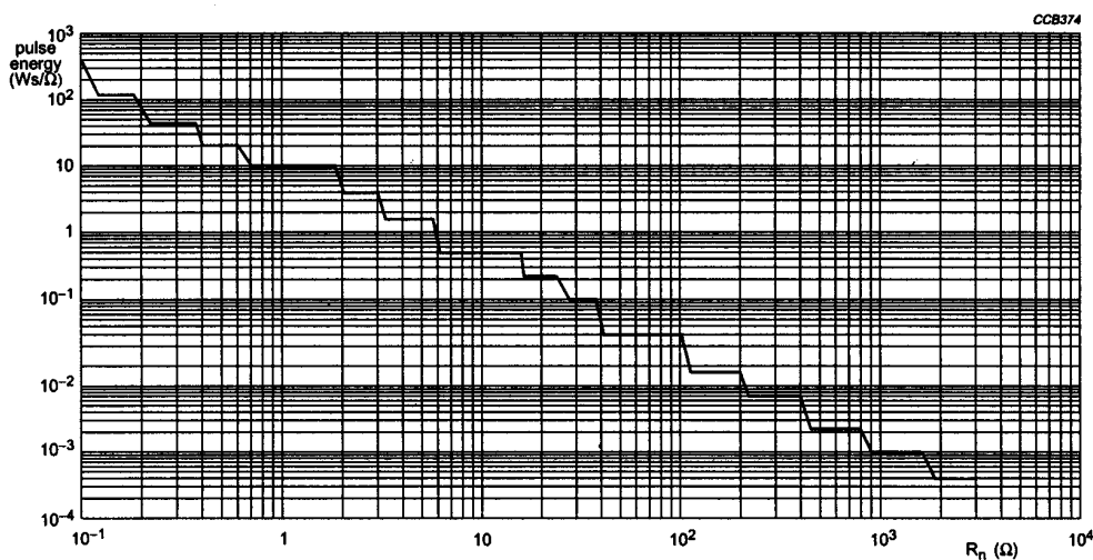
Fig. 19 Pulse capability; Ws as a function of Rn
