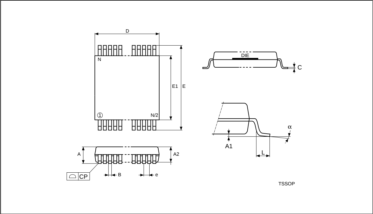
Figure 18. TSSOP14 (DL)
