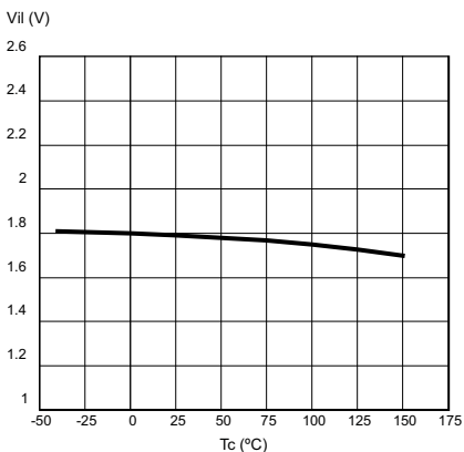
Figure 10. Input low level voltage
