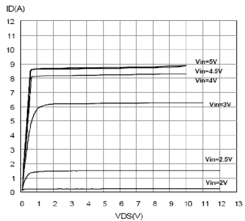
Figure 33. Output characteristics
