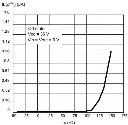
Figure 6. Off-state output current
